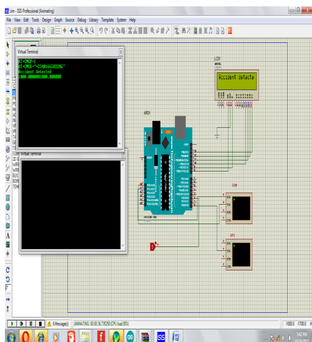
Fig. 9: Simulation result showing accident is detected
