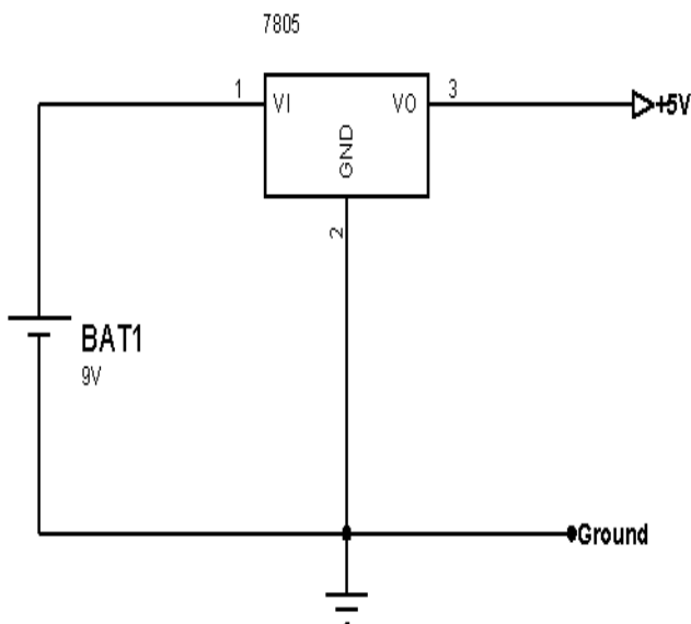
Fig. 2: Power supply unit circuit
