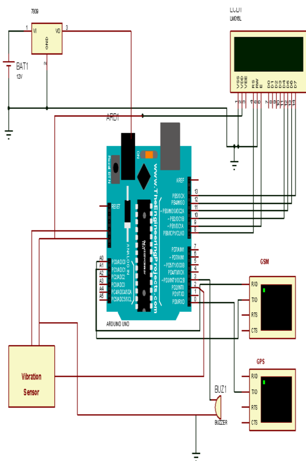
Fig. 6(a): Complete circuit diagram
