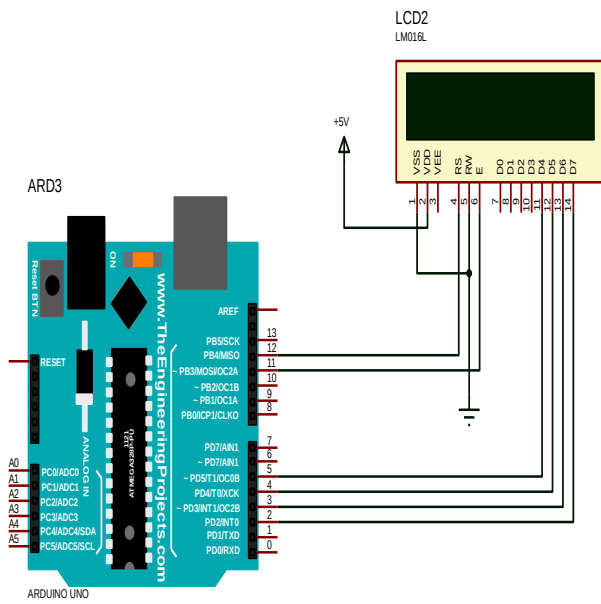
Fig. 4: Arduino to LCD Interfacing
